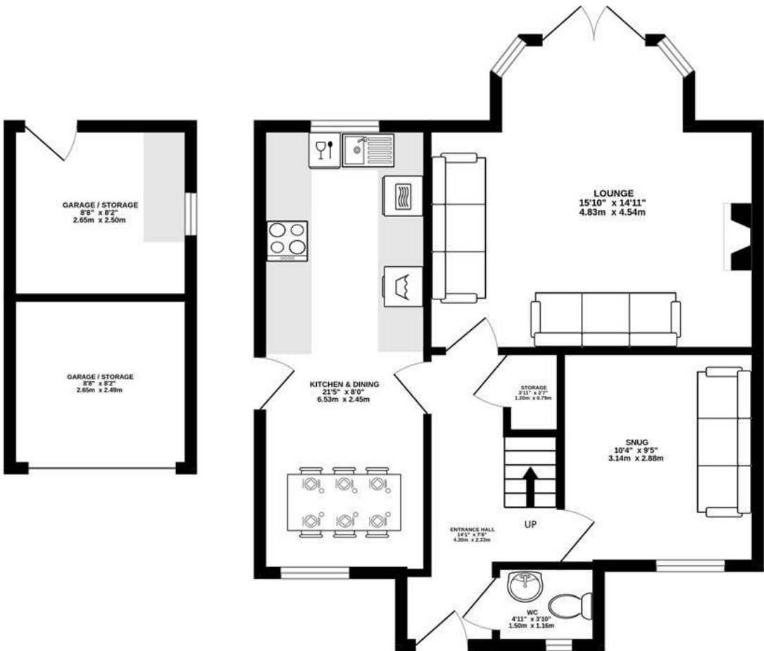
GROUND FLOOR 715 sq.ft. (66.5 sq.m.) approx.
